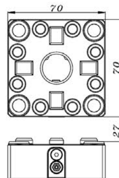
品名: 70方型手動單頭卡盤(螺絲鎖緊) 70 mm square Manual Marco Chuck (screw locking)
