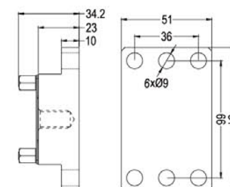
品名: 81x51平面不銹鋼夾頭 81x51 FLAT STAINLESS STEEL HOLDER
