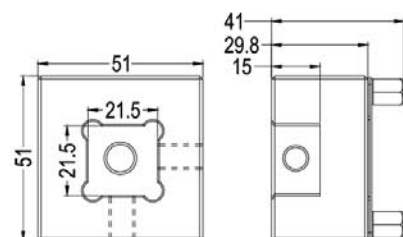
品名: S20方型不銹鋼夾頭 S20 STAINLESS STEEL HOLDER
