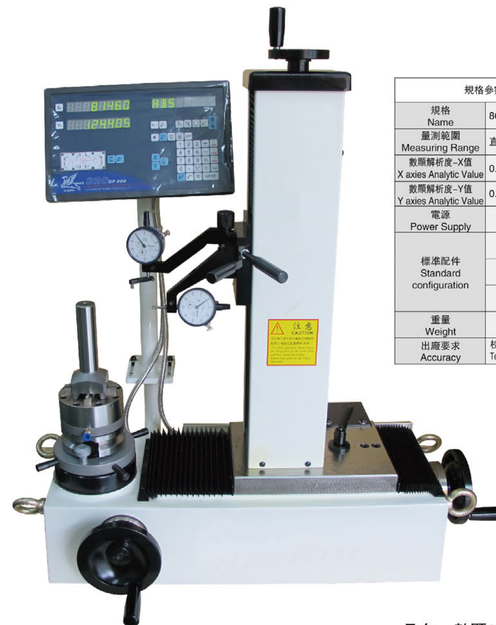
品名：數顯2軸夾具預調儀 3D Workpiece Detector
