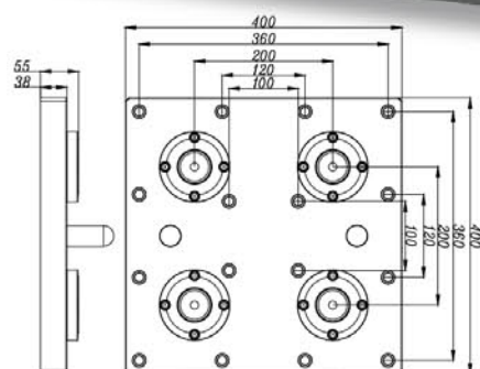
品名: 4頭重力型卡盤面板 4 Heads Heavy Duty Pneumatic Pallet (Use With PO-J0004)
