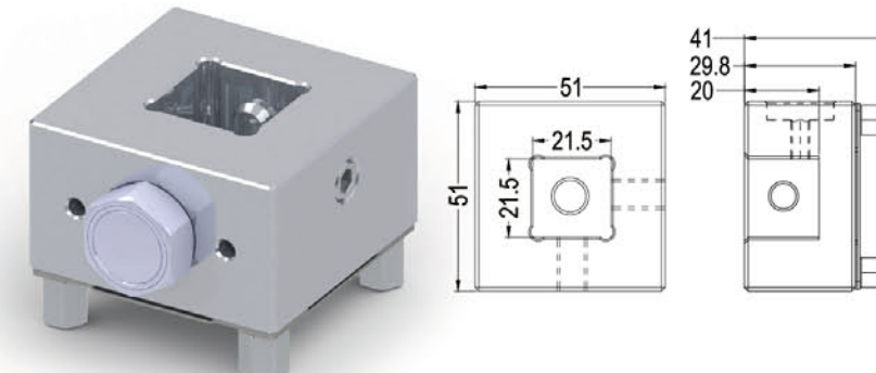
品名: S20槽型鋁合金夾頭 S20 ALUMINUM HOLDER
