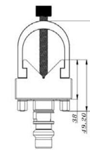
品名：V型座線切割夾頭 V-Shape Wire Cut EDM Holder
