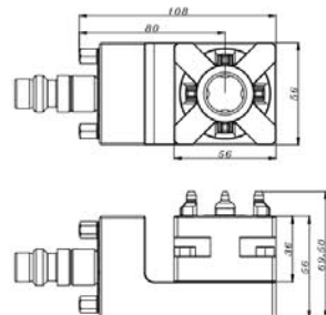
品名：小型轉向EDM手動卡盤(手柄鎖緊) Vertical EDM Quick Chuck 50
