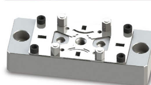
品名: 130x51平面不銹鋼夾頭 130x51 FLAT STAINLESS STEEL HOLDER
