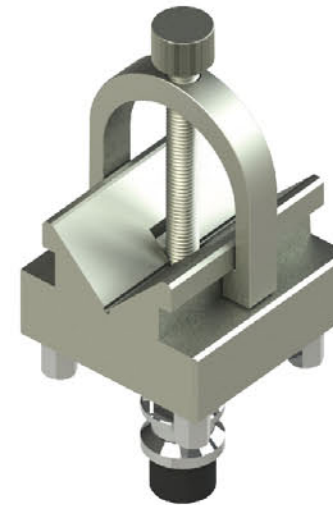
品名：V型座線切割夾頭 V-Shape Wire Cut EDM Holder
