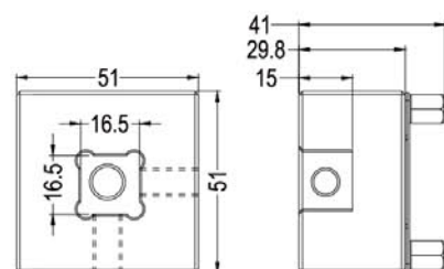
品名: S15方型不銹鋼夾頭 S15 STAINLESS STEEL HOLDER
