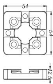
品名: 54x54定位片 3M Centering Plate 54x54
