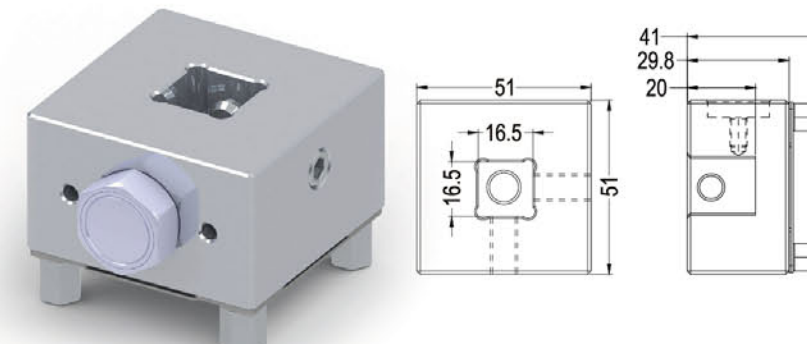
品名: S15槽型鋁合金夾頭 S15 ALUMINUM HOLDER
