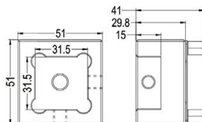
品名: S30方型不銹鋼夾頭 S30 STAINLESS STEEL HOLDER
