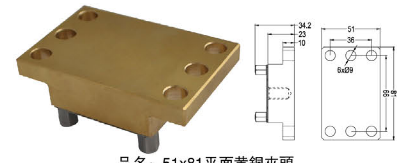
品名: 51x81平面黃銅夾頭 51x81 FLAT BRASS HOLDER
